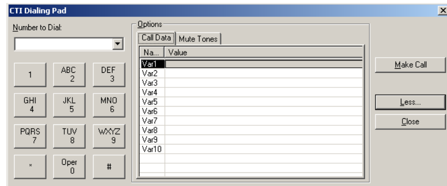
Figure 5-24 Expanded Dialog
