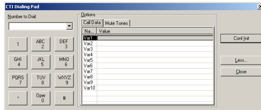
Figure 5-17 Expanded Dialog
