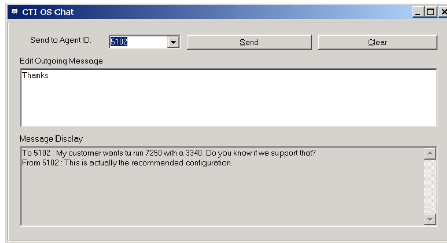
Figure 5-13 Chat Control
