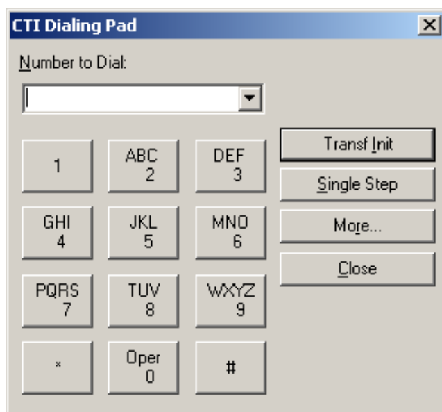
Figure 5-28 Dial Dialog
